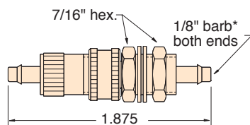
Part No. MIQC-PBB4 Description 1/8" Barb Outlet, 1/8" Barb Inlet with Thread (MJQC-VB4/MJQC-CPB Combo) (supplied with mounting nut and two washers)
