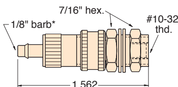
Part No. MIQC-PFB4 Description 1/8" Barb Outlet, #10-32 Inlet (MJQC-VB4/MJQC-CPF Combo) (supplied with mounting nut and two washers)
