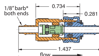
Part No. MIQC-B4B4 Description 1/8" Barb Outlet, 1/8" Barb Inlet (MJQC-VB4/MJQC-CB4 Combo)
