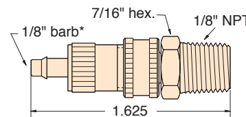
Part No. MIQC-MPB4 Description 1/8" Barb Outlet, 1/8" NPT Inlet (MJQC-VB4/MJQC-CMP Combo)
